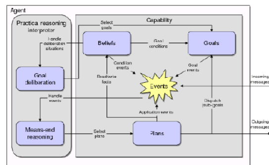
Fig 7: BDI agent working process
