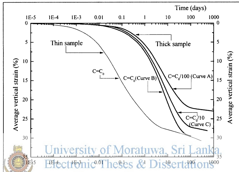
Fig. 4.7: Numerical simulation of the effect of sample thickness on settlement predictions
