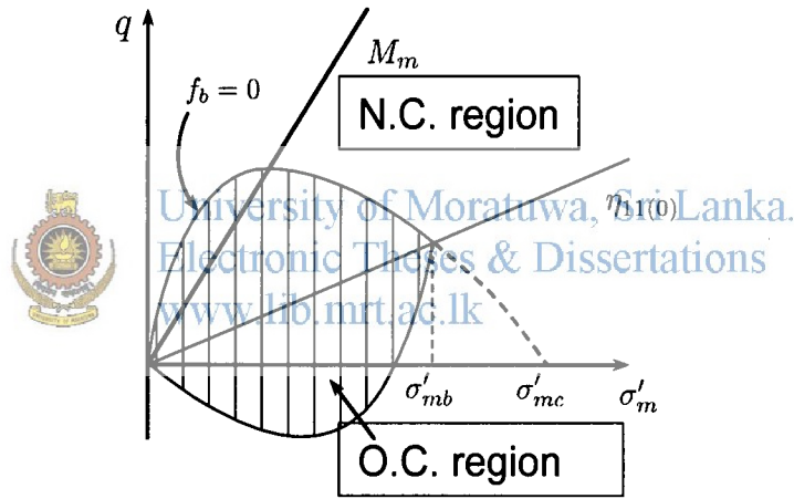
Fig. 3.2: Overconsolidated boundary surface under triaxial conditions (Kimoto 2002)
