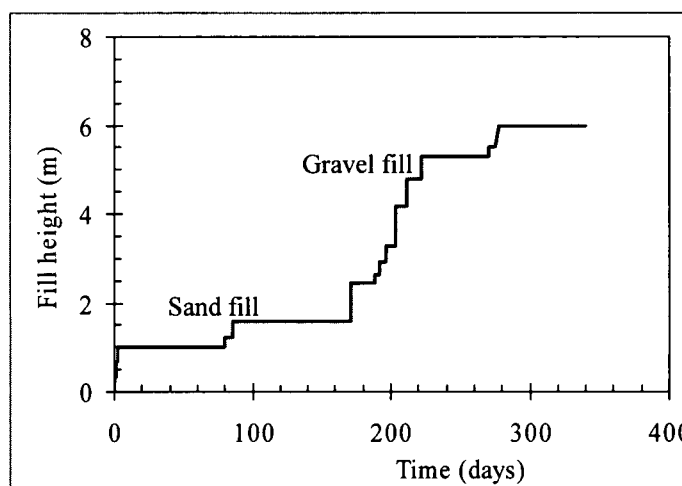
Fig. 6.2: Loading curve
