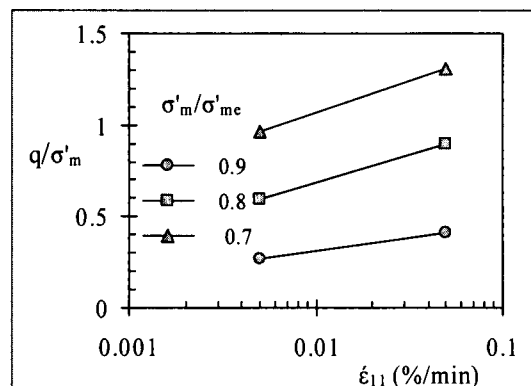
Fig. 4.15(d): q/\sigma'_m vs. \dot{\epsilon}_{11} relationship
