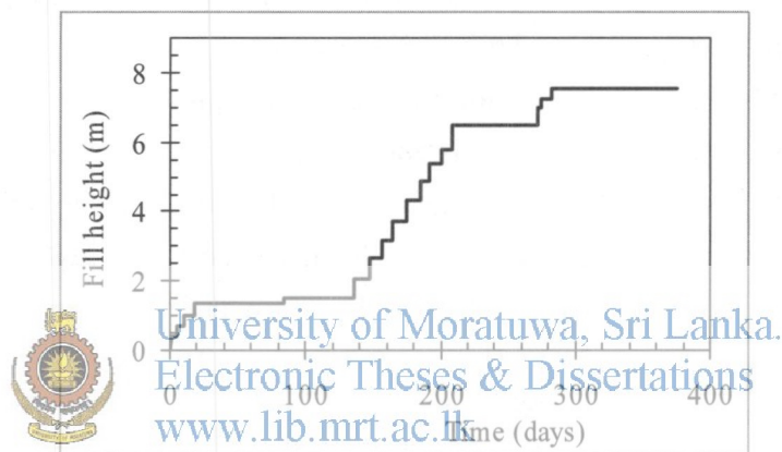
Fig. 7.16: Loading curve
