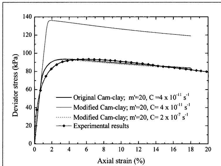
Fig. 3.10: Comparison of the stress-strain behavior University of Moratuwa, Sri Lanka. Electronic Theses & Dissertations www.lib.mrt.ac.lk
