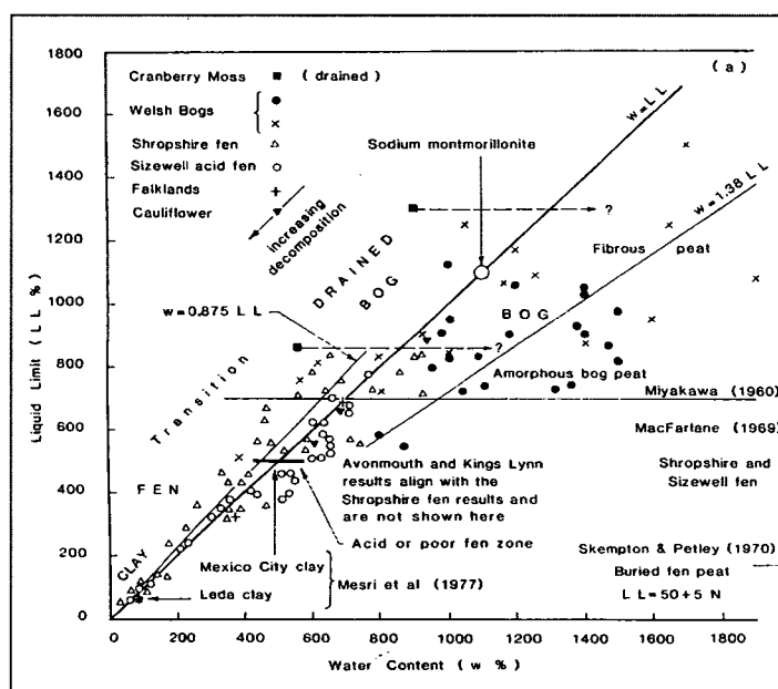
Fig. 2.4: Liquid limit vs. water content relationship for peats (Hobbs 1986)
