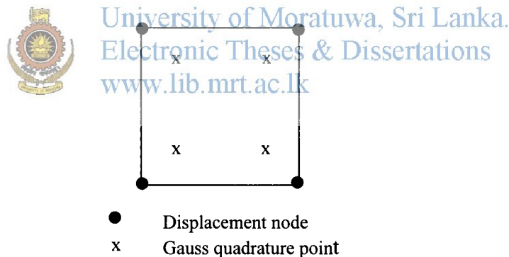
Fig. 5.11: Four-node isoparametric element for displacement interpolation
