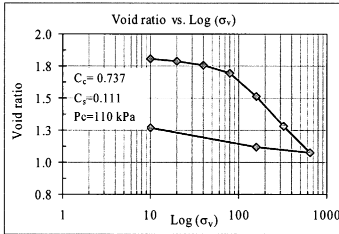
Fig. 4.15(a): Void ratio vs. Log (stress) relationship
