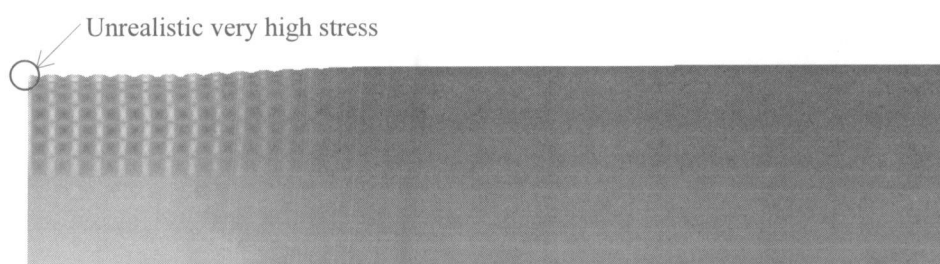
Fig. 7.20 Mean effective stress distribution in the foundation due to embankment loading (kPa)
