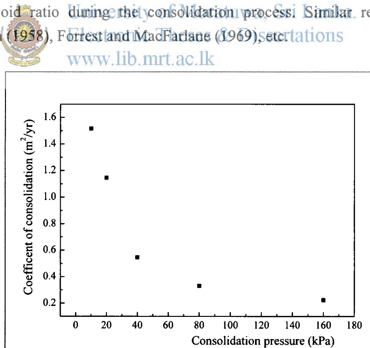
Fig. 1.3: Variation in coefficient consolidation during the consolidation process
