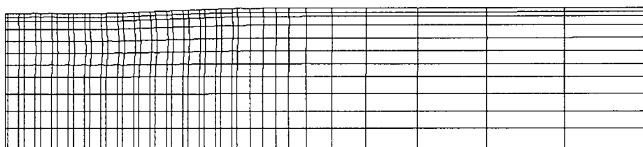
Fig. 7.22: Predicted deformation pattern for the embankment at the end of construction
