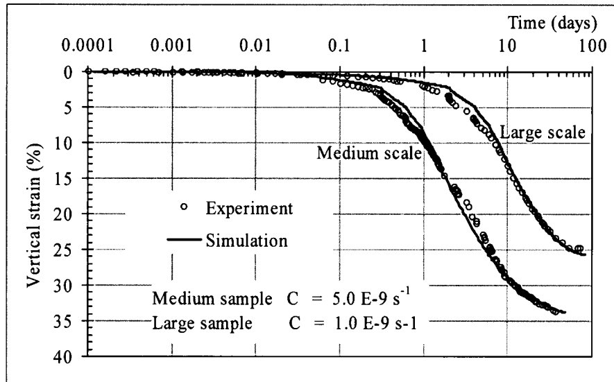
Fig. 4.11: Strain predicted by considering the difference in initial strain rates
