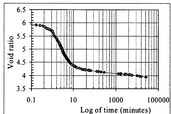
Fig. 4.2: Void ratio vs. \text{Log}(\text{time}) relationship
