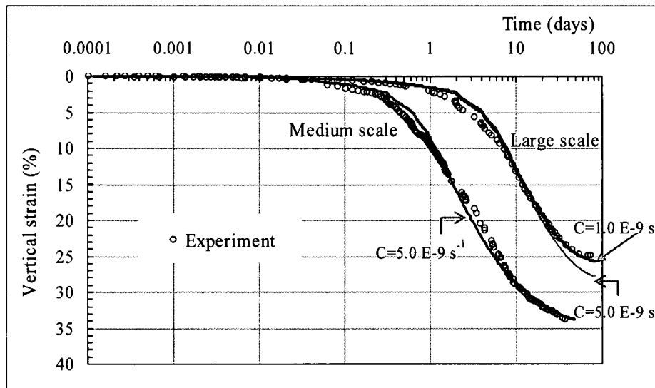
Fig. 4.12: Strain predicted by considering the same initial strain rates for the thick and the thin samples
