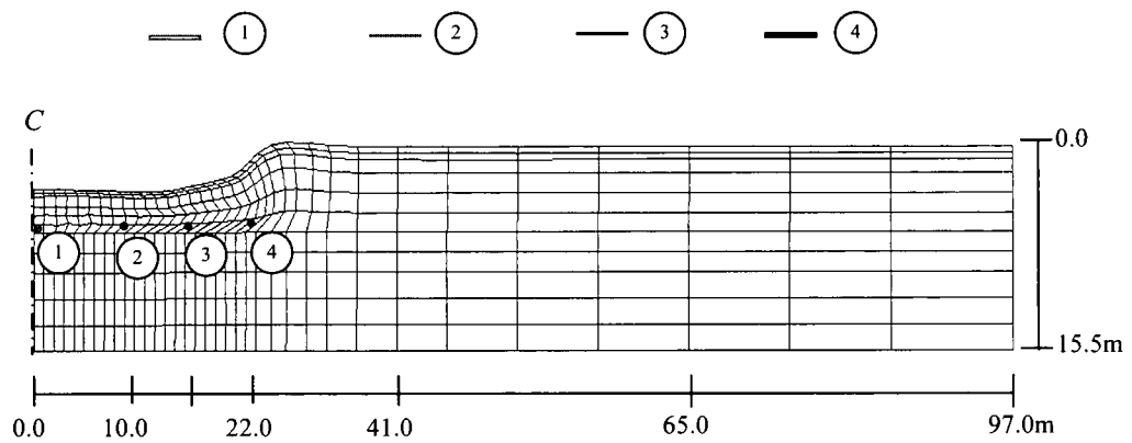
Fig. 6.10: Soil element behavior under the embankment – silty clay/ peat 5.75 m depth
