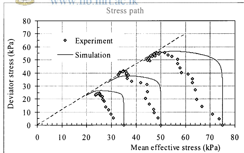
Fig. 5.9: Simulation of the stress paths
