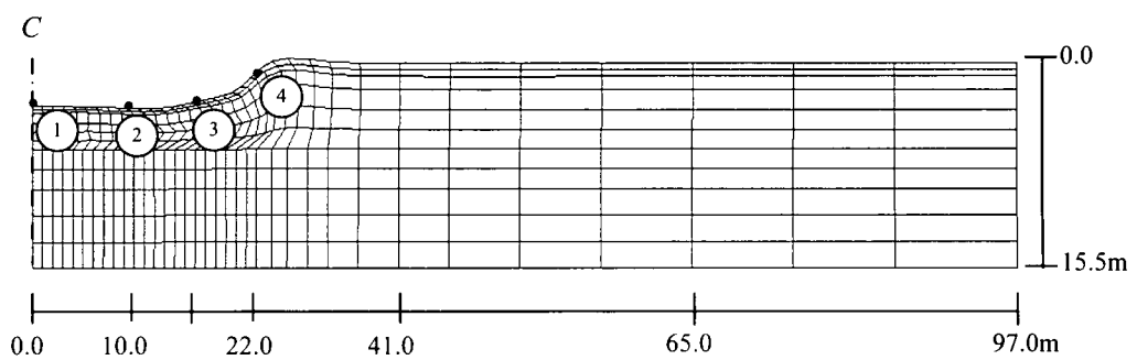
Fig. 6.15: Soil element behavior under the embankment – peat 0.25m depth
