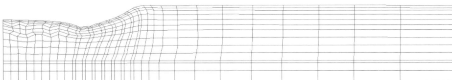
Fig. 7.28: Deformation pattern of the embankment foundation without considering SCP improvement under the slope
