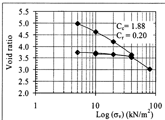
Fig. 4.1: Void ratio vs. \text{Log}(\sigma'_v) relationship
