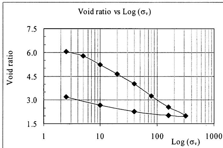
Fig. 3.5: Typical e - \log \sigma_v curve for Sri Lankan
