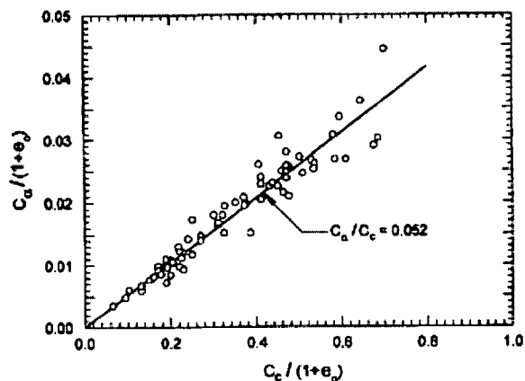
Fig. 2.7: C_\alpha/C_c relationship for Middleton peat, UK (Mesri et al.1997)
