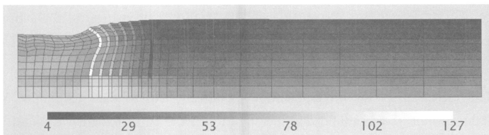
Fig. 7.27: Distribution of mean effective stress for embankment foundation (kPa)
