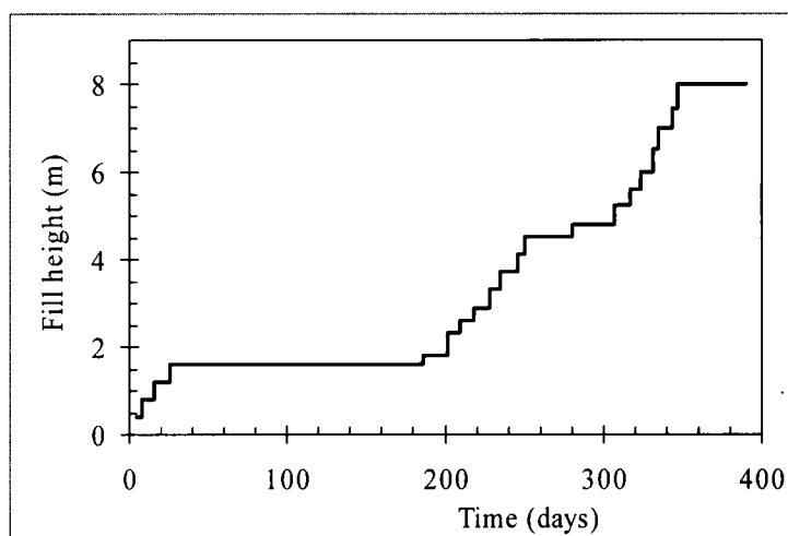
Fig. 7.5: Loading curve
