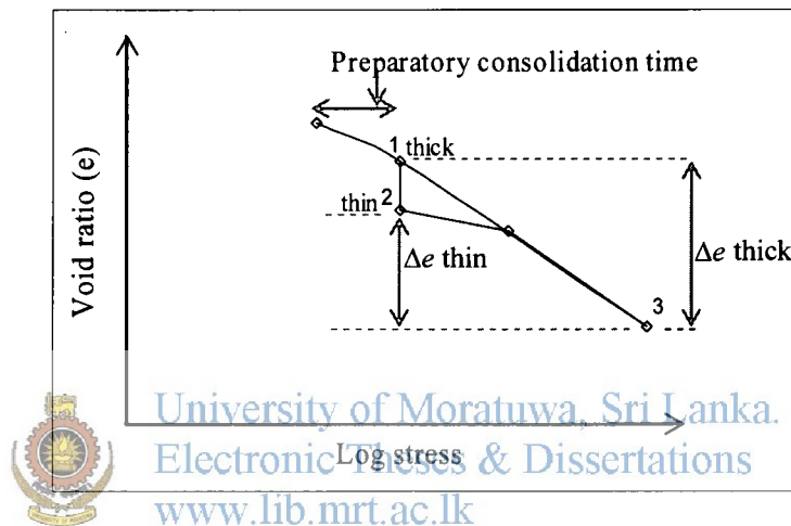
Fig. 4.9: Importance of controlling the preparatory consolidation time
