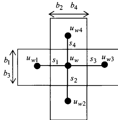
Fig. A1.1: Drainage distance used to evaluate the rate of flow (Tamura 1979)
