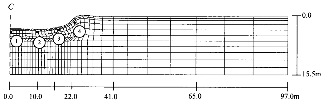
Fig. 6.13: Soil element behavior under the embankment – silt 1.5 m depth
