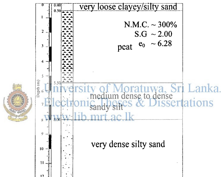
Fig. 5.4: Subsurface profile at the site
