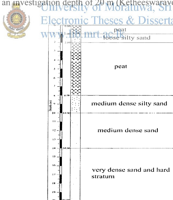
Fig. 7.15: Subsurface profile at the site
