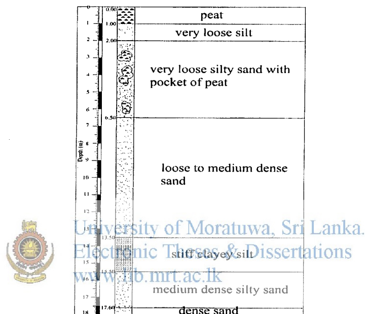
Fig. 6.1: Subsurface profile beneath the embankment (Ketheeswaravenavagam 2006)
