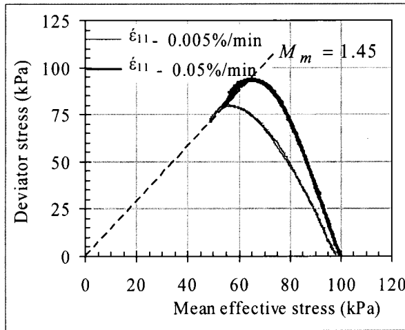
Fig. 3.8: Stress paths
