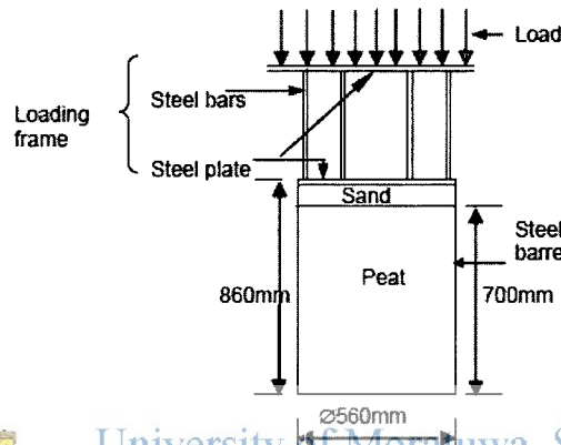
Fig. 4.8: Schematic diagram of the large scale model
