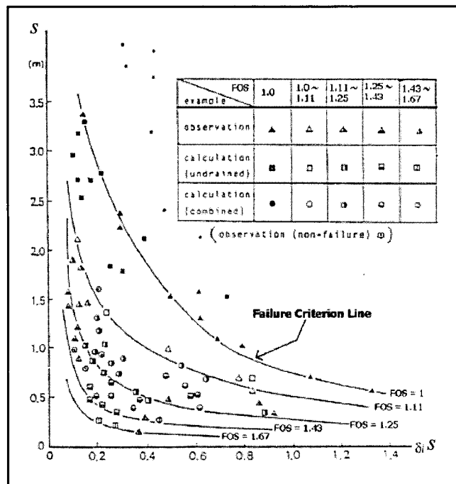
Fig. 7.12: Modified Matsuo stability plot
