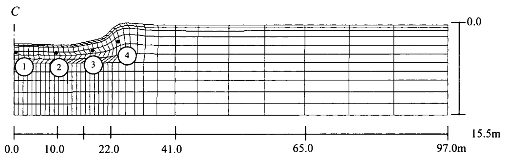
Fig. 6.12: Soil element behavior under the embankment – silty clay/peat 2.75 m depth
